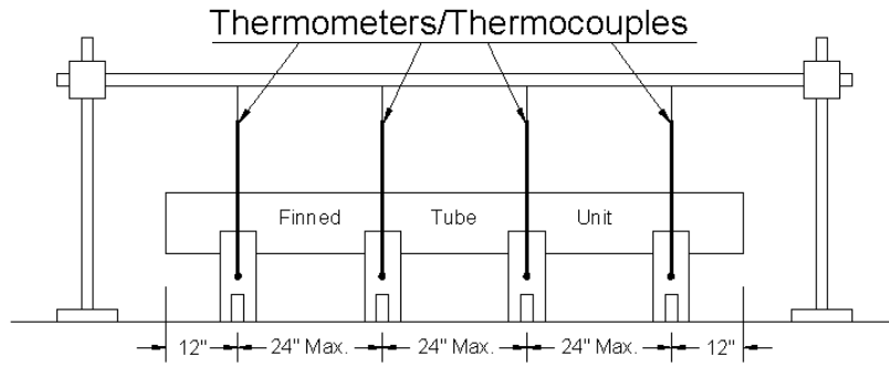
Figure C3. Location of Thermometers/Thermocouples in Front of the Test Unit
