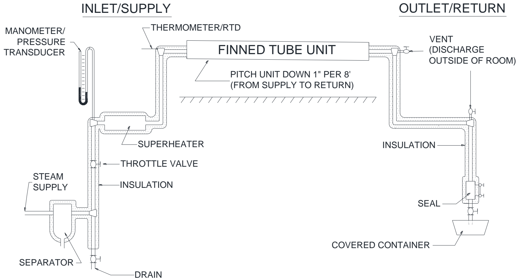
Figure C5. Suggested Methods and Equipment for Supplying Steam to the Finned Tube Unit and Measuring the Condensate
