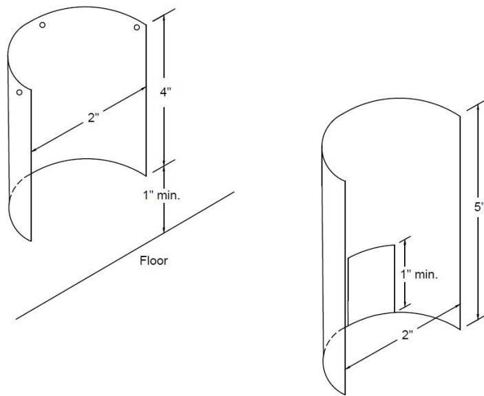
Figure C4. Suggested Construction of Thermometer/Thermocouple Shield of Bright Metal
