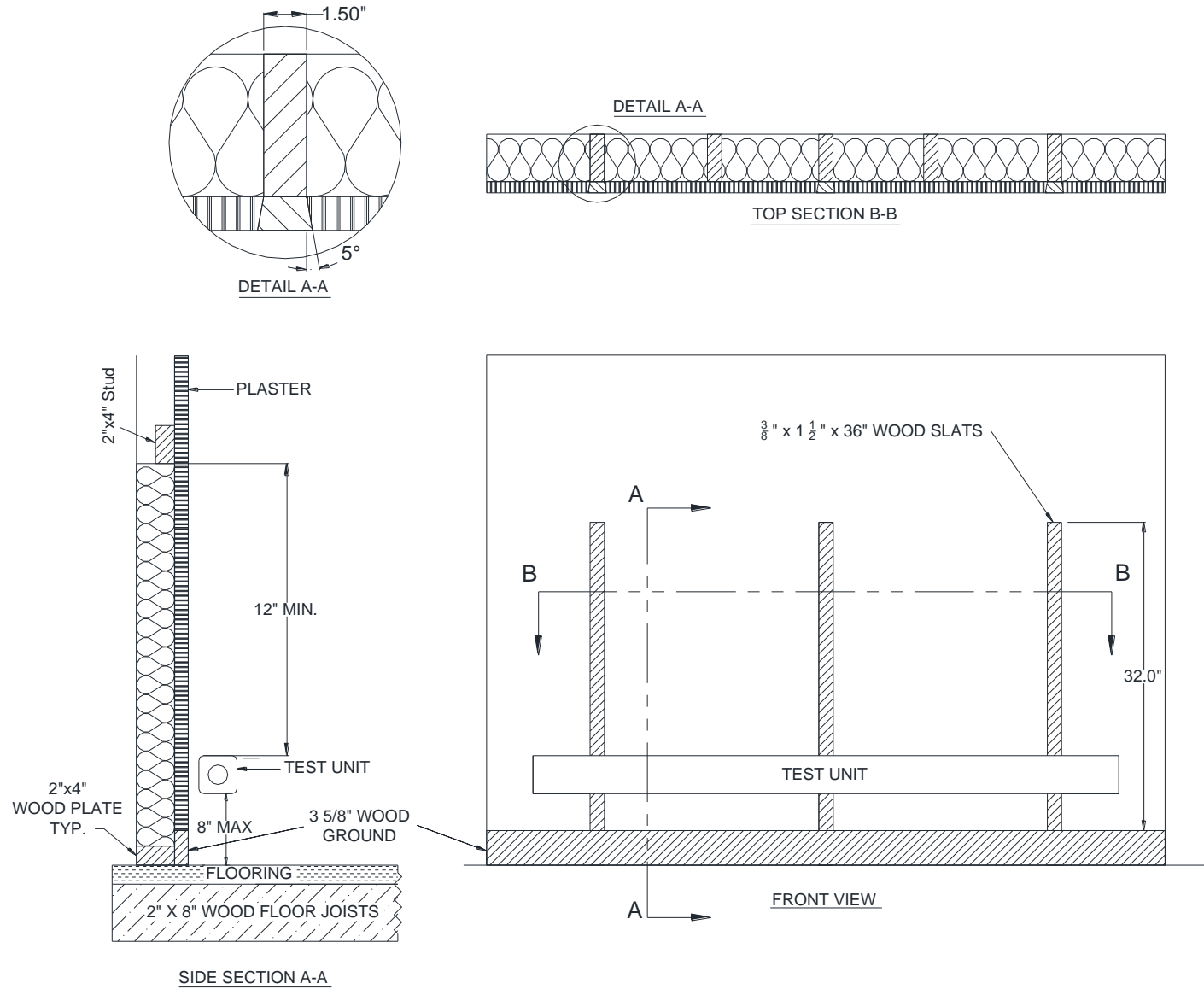
Figure C1. Test Unit Wall Construction
