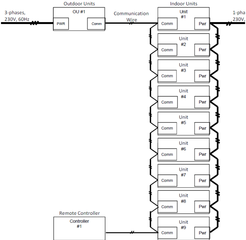
Figure D1. Example Wiring Diagram for Heat Pump
