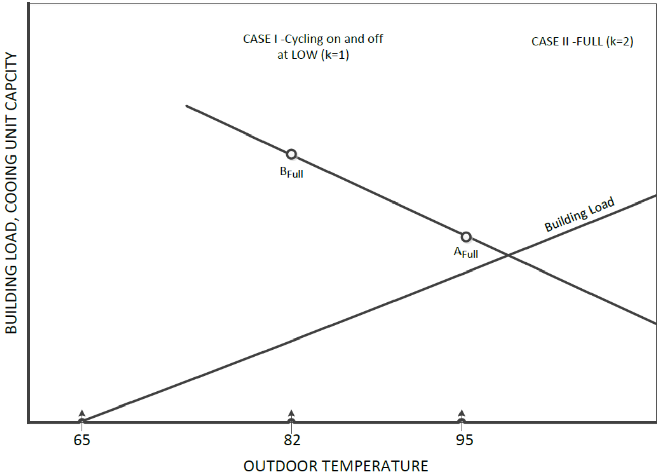
Figure 2. Schematic of a Single-speed System Operation in the Cooling Mode (See Tables 8 and 9 for Temperature References)
