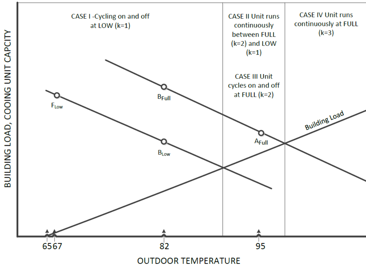
Figure 4. Schematic of a Two-speed System Operation in the Cooling Mode (See Tables 8 and 9 for Temperature References)
