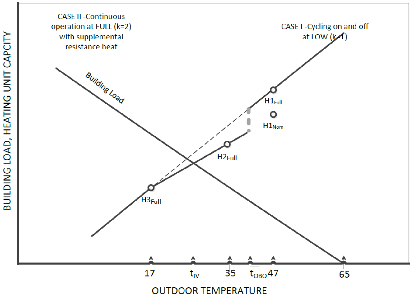
Figure 7. Schematic of a Single-speed Heat Pump Operation in Heating Mode
