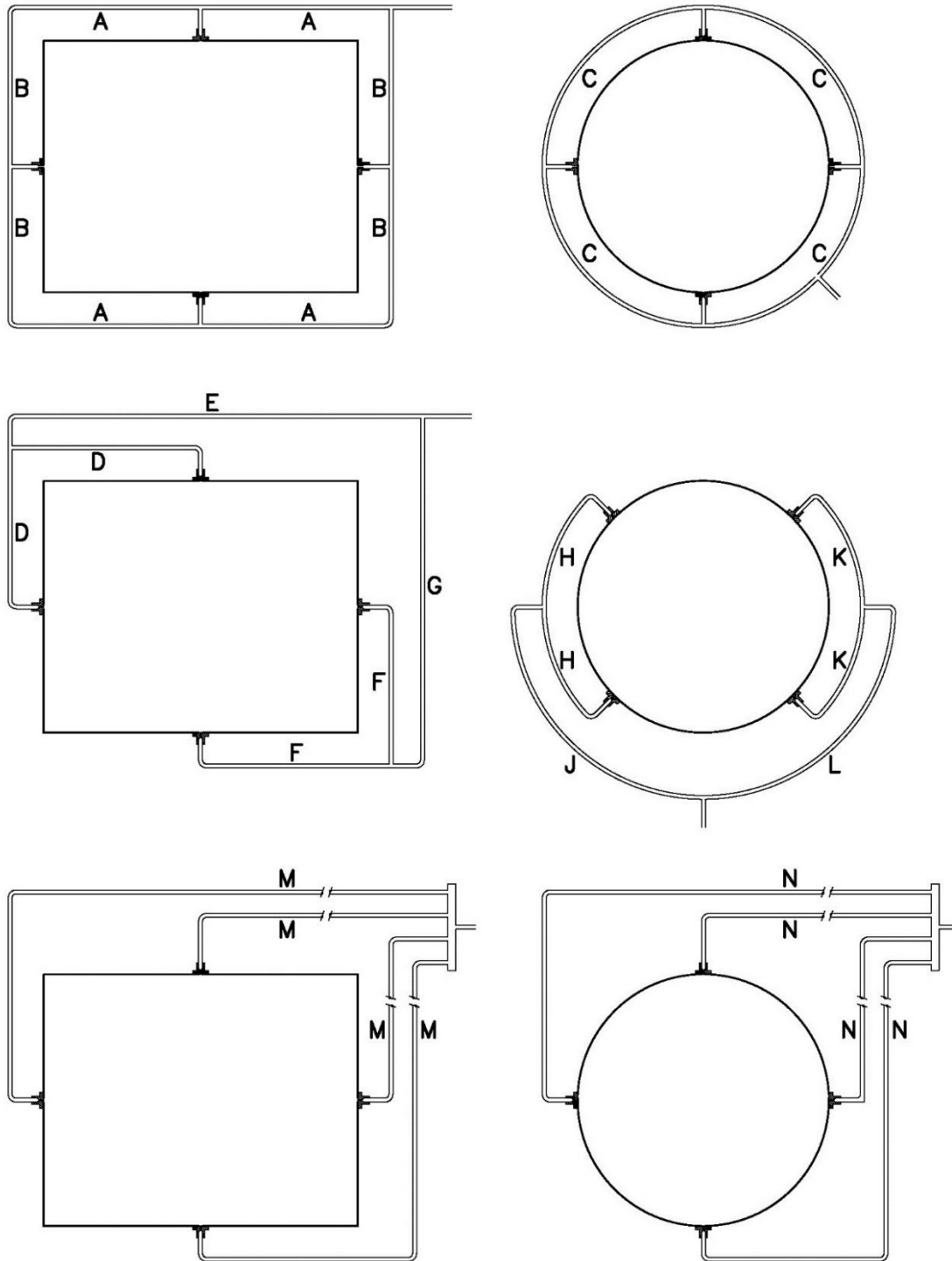
Figure E1. Configurations for Manifolding the Static Pressure Taps
