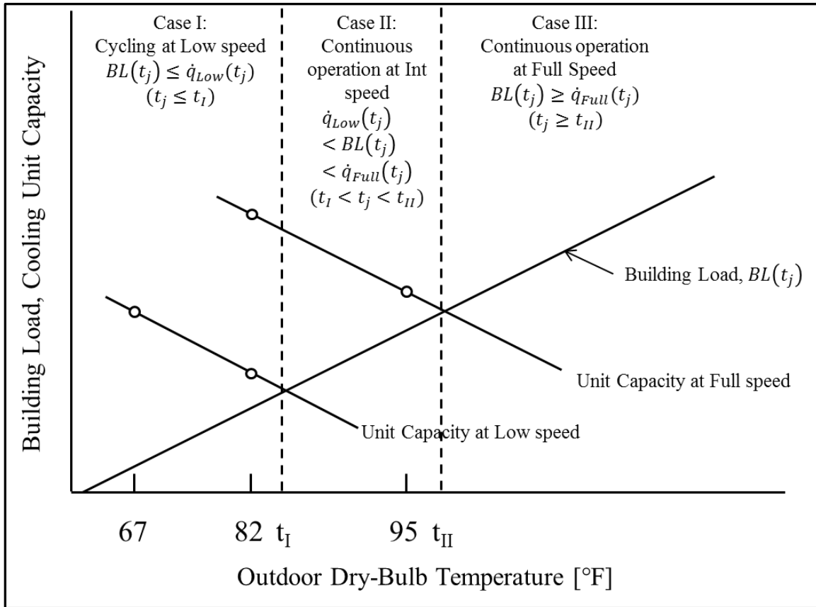
Figure 5. Schematic of a Variable Speed System Operation in the Cooling Mode
