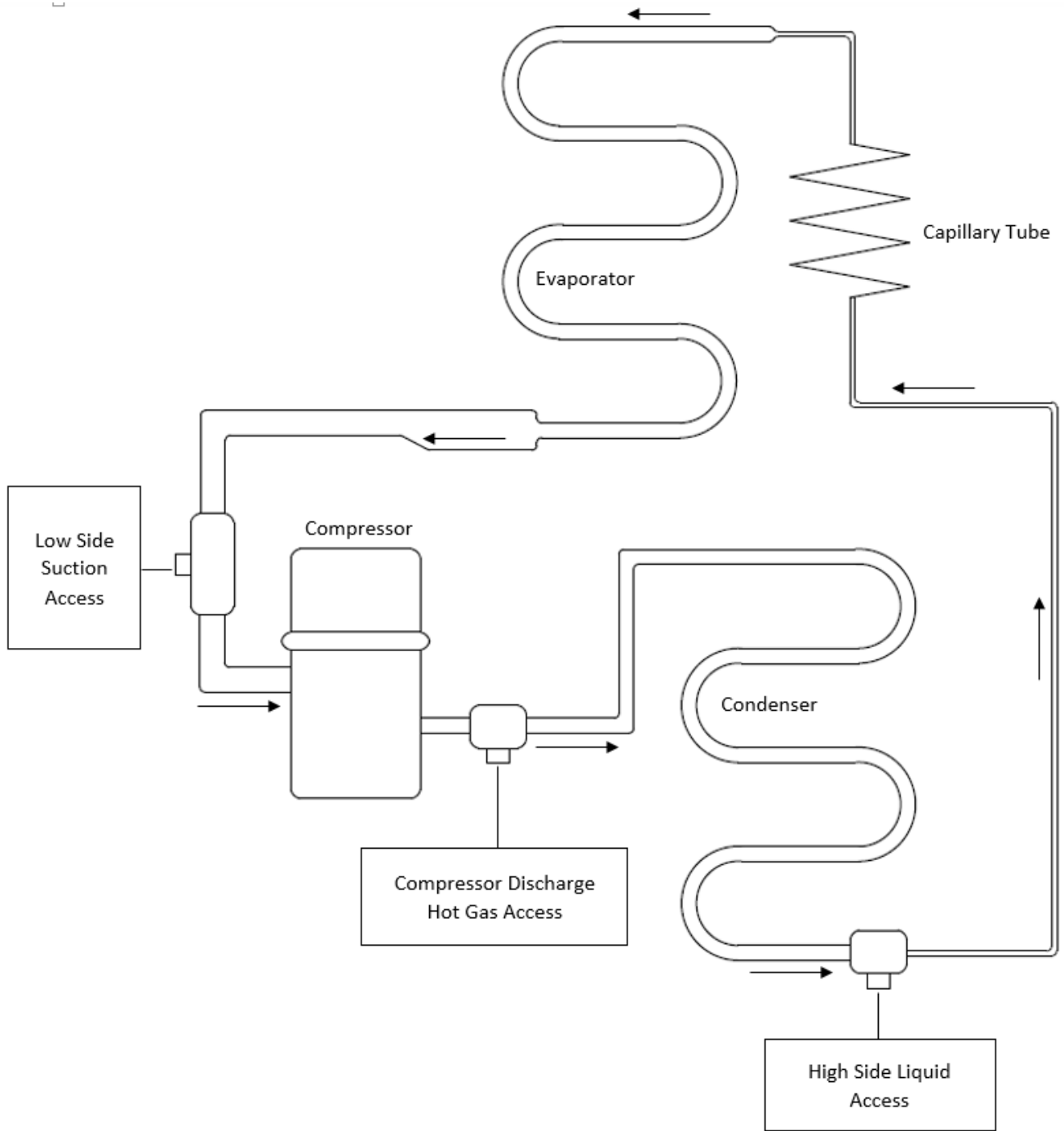
Figure C2. System Dependent Equipment Test Apparatus
