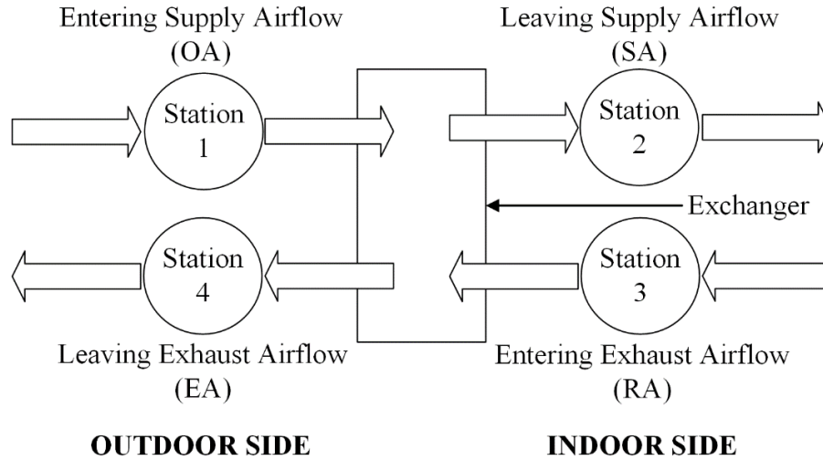
Figure 1. Scheme of Airflows for Exchangers
