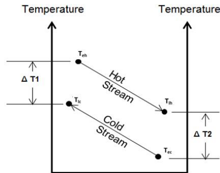
Note: If \Delta T1 = \Delta T2 , LMTD = \Delta T Figure D1. Counter Flow
