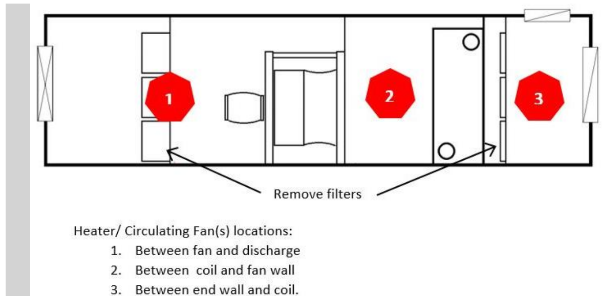
Figure C15. CSAHU with Pressure Change Wall
