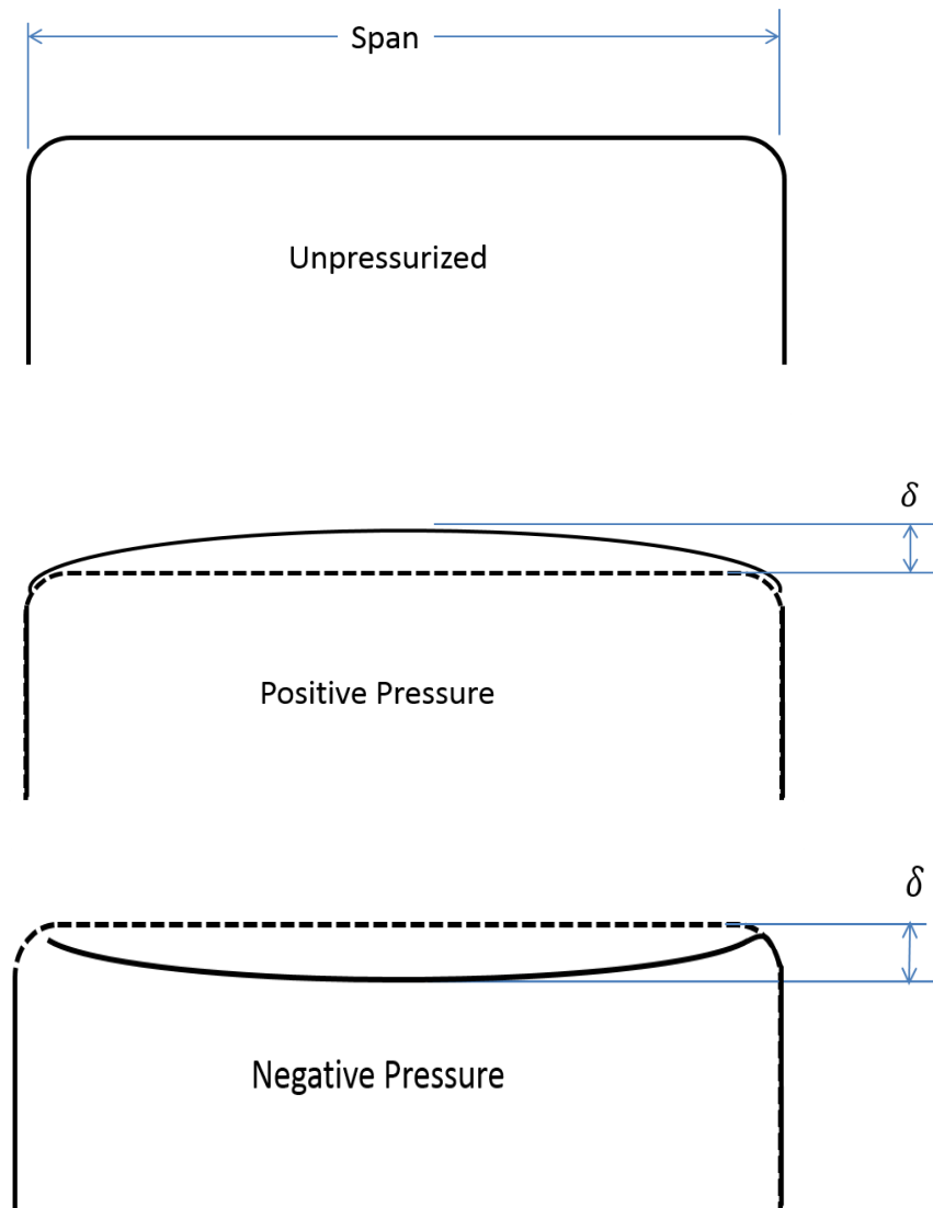
Figure C7. Deflection Measurement
